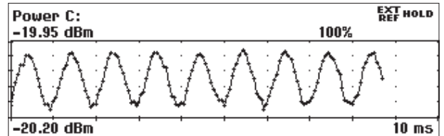
Fig. 4: Very small AM on carrier is visualized
