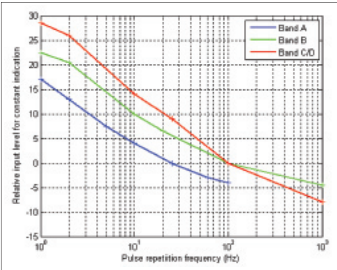
Figure 7. Pulse response curve with a Quasi-peak detector.
