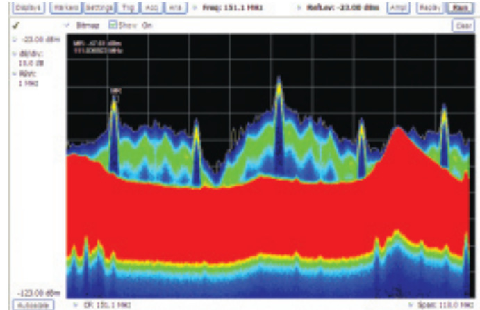
Figure 11. Infrequent transient discovered with DPX after 5 seconds. The red areas are frequently-occurring signals, and the blue and green portions are transients.
