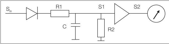
Figure 5. Quasi-peak detector in an analog implementation. The fast-attack (charge time) and slow-decay (discharge time) of the quasi-peak detector result from the R-C constants implemented in this circuit. The resultant waveform drives the critically-damped meter.
