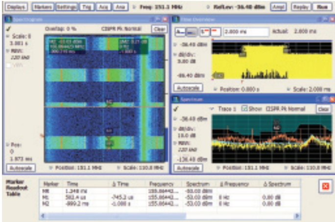
Figure 12. The transient that occurs at 1 second repetition rate is captured using a frequency mask trigger.
