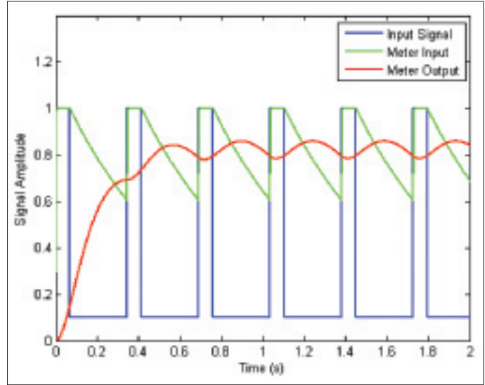
Figure 6. Quasi-peak response to a repetitive signal.
