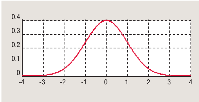
Figure 4.2.1a. Gaussian Distribution.
