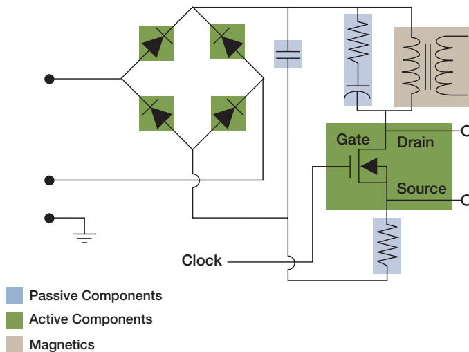
Figure 1. Switch-mode power supply simplified schematic.
