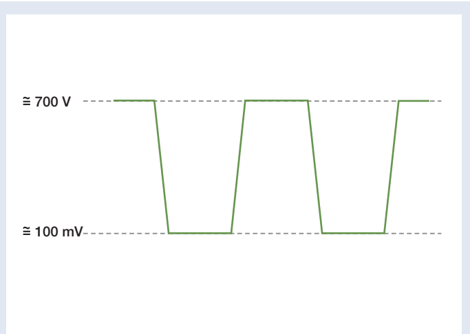
Figure 6. Typical signal of a switching device.
