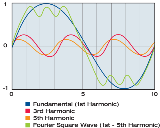
Figure 15. Harmonic contributions to square wave makeup.
