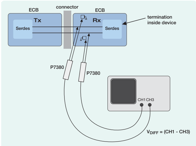
Figure 8. Pseudo-differential probing of a receiver input.
