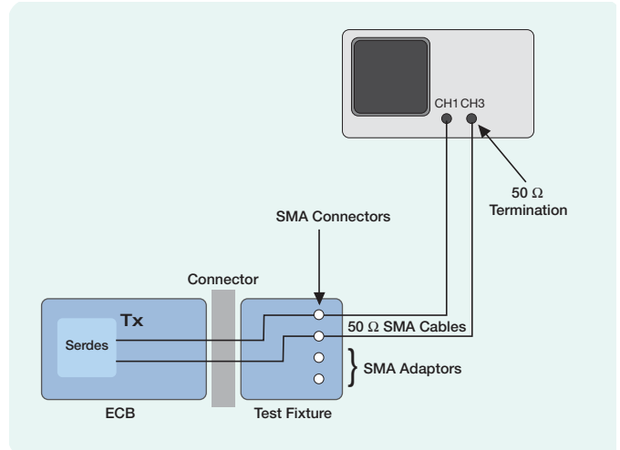
Figure 9. Pseudo-differential connection to a fixture using SMA-terminated cables.
