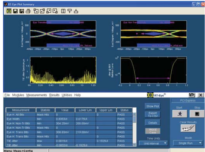
Figure 13b. Receiver testing with FIR filtering.
