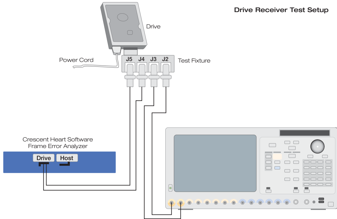
Figure 14. Receiver jitter measurement setup.
