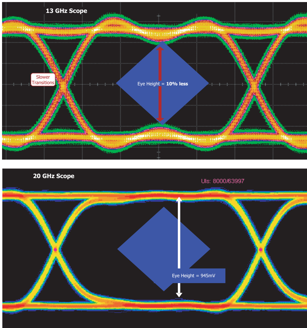
Figure 16. Effects of oscilloscope bandwidth on eye analysis.
