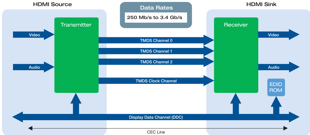
Figure 3. HDMI architecture.
