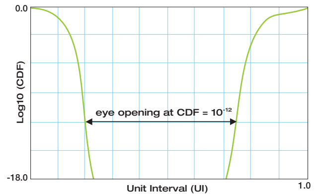
Figure 19. Jitter bathtub curve.
