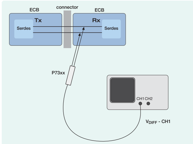
Figure 10. True differential probing of a receiver input.
