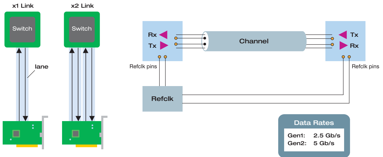
Figure 2. PCI Express architecture.
