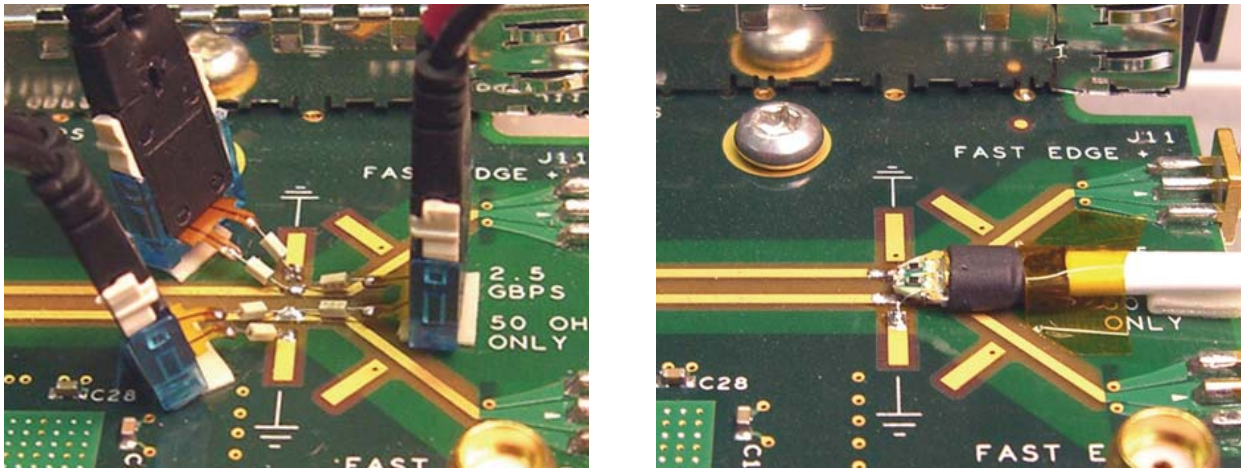
Figure 7a/7b. Tri-mode probes (right) simplify test traditional setups (left) and measurements.
