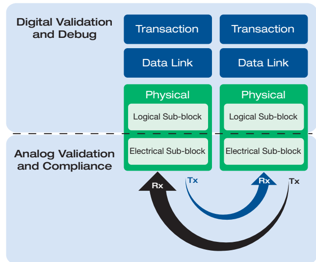
Figure 4. Layered model.
