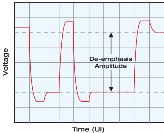
Figure 6. De-emphasis on a data stream.
