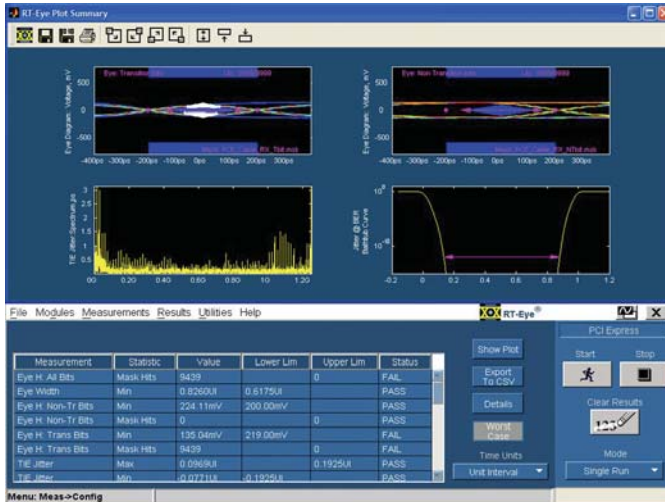
Figure 13a. Receiver testing without FIR filtering.
