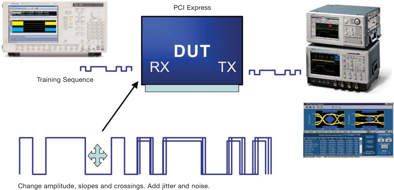
Figure 12. PCI Express receiver testing setup.
