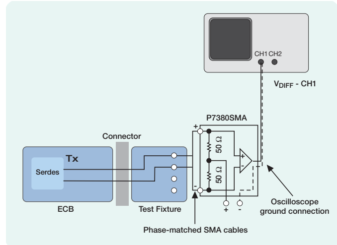
Figure 11. Differential connection on a fixture using SMA-terminated cables.
