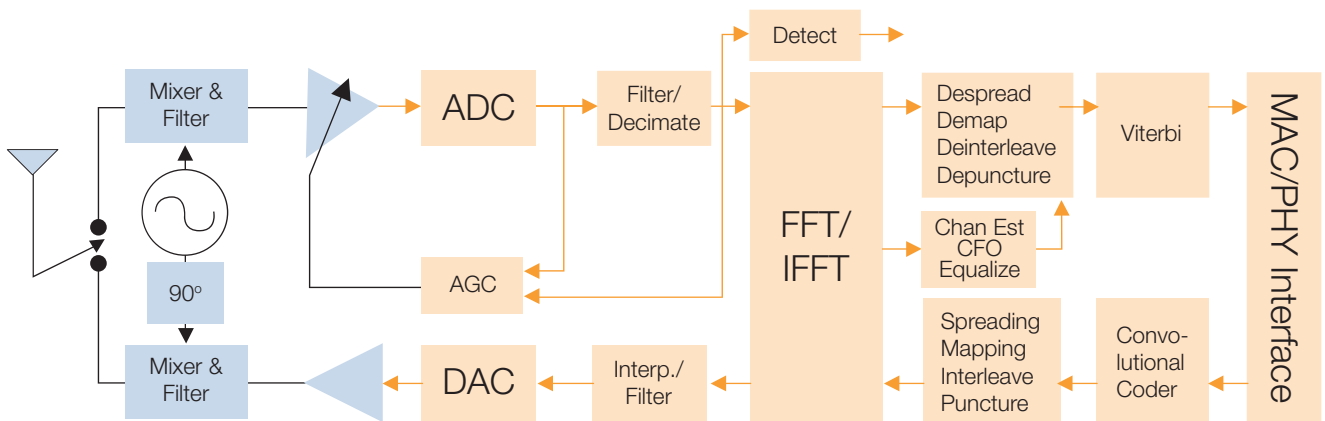
Figure 3. Block diagram of a UWB Tx / Rx.
