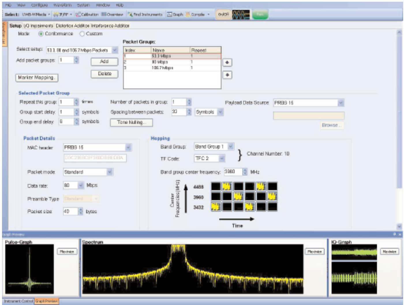
Figure 1. RFXpress in conformance mode. RFXpress is a software package to synthesize digitally modulated baseband. IF and RF signals which can be generated with Tektronix AWG7000 Series arbitrary waveform generators (AWGs).
