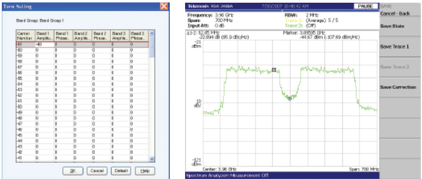
Figure 15. Tone nulling.
