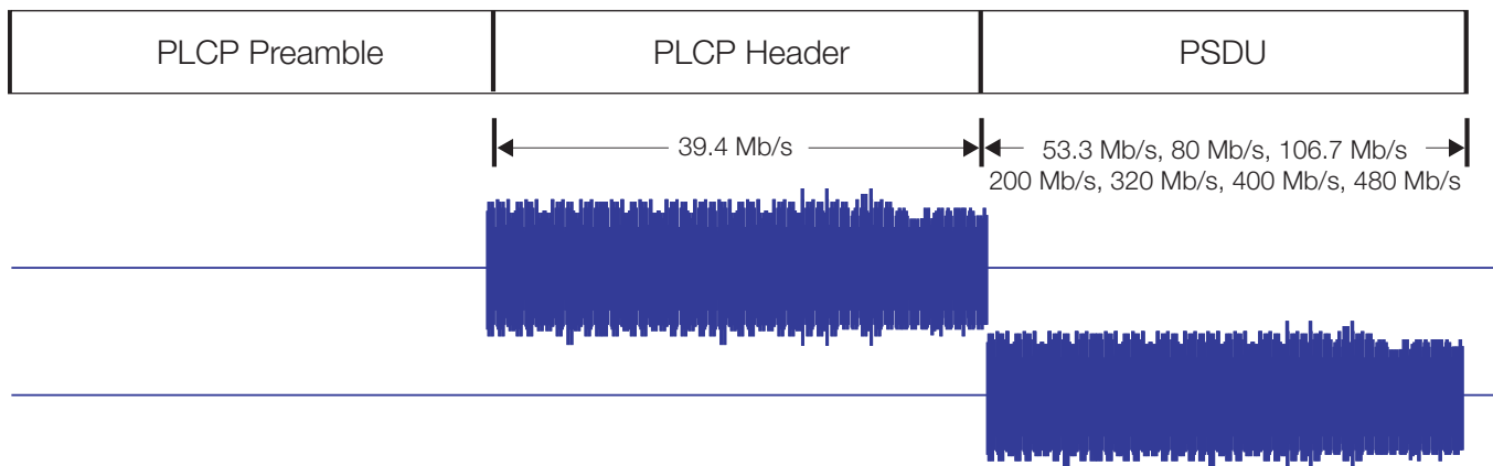
Figure 16. Symbolic representation of gated noise.
