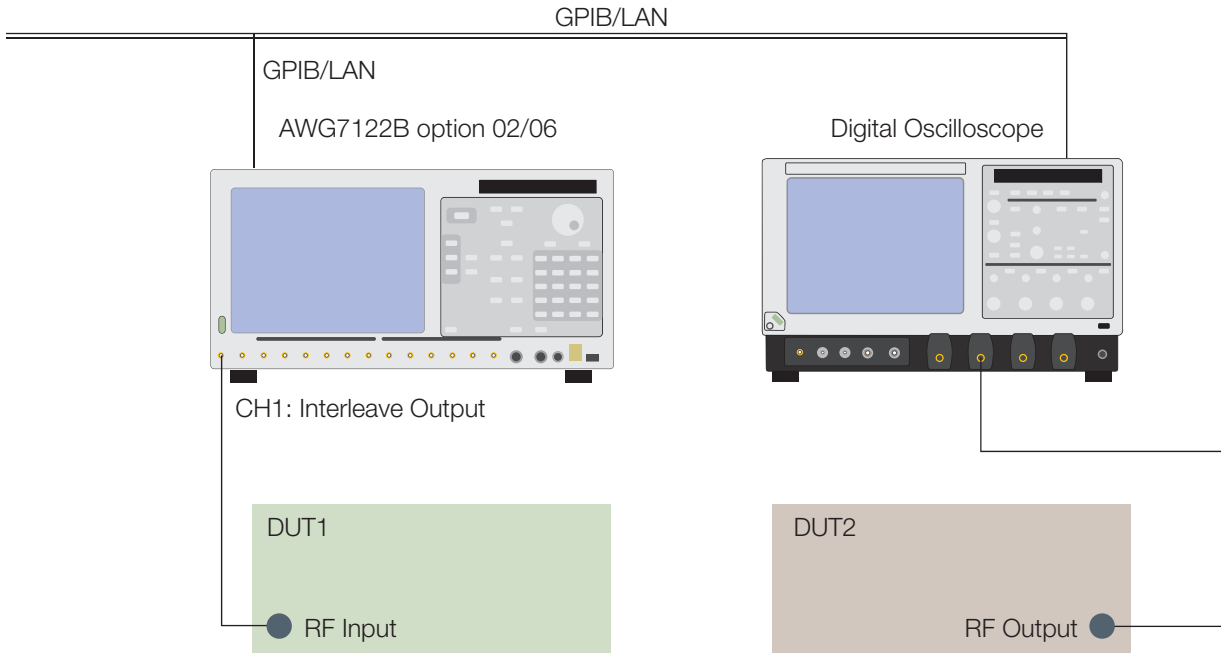
Figure 14. Connect, capture and reply a waveform from an oscilloscope.
