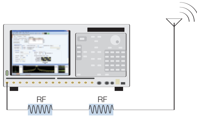
Figure 6. WiMedia direct RF signal generation using an AWG and RFXpress software. External PC not required.
