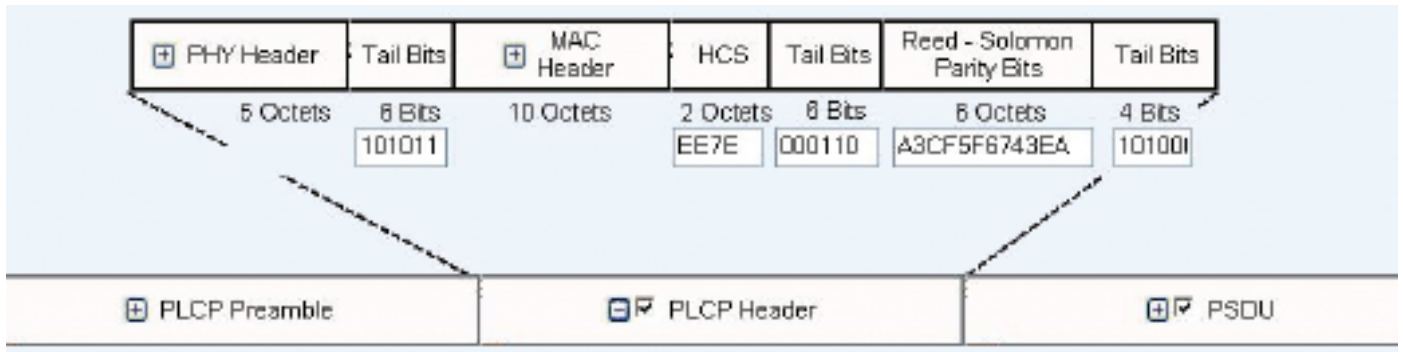
Figure 8. PDU structure.
