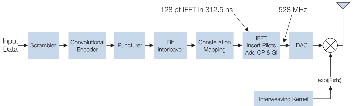
Figure 2. UWB WiMedia Tx chain.
