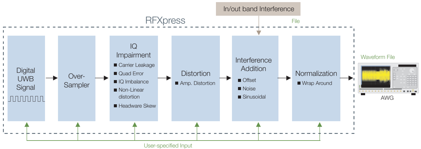
Figure 12. RFXpress signal flow chart.
