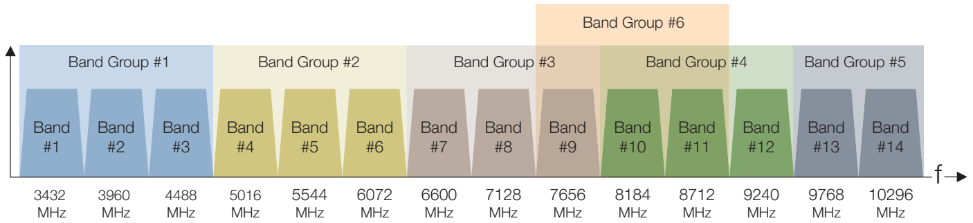
Figure 4. WiMedia band groups.
