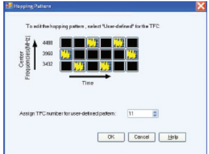
Figure 11. User defined TFC in RFXpress custom mode.
