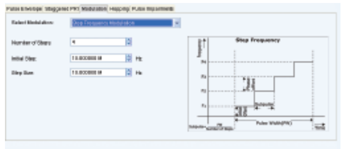
Figure 13. An illustration of Step Frequency Modulation.
