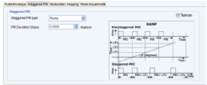
Figure 12. A staggered PRI with Ramp type.
