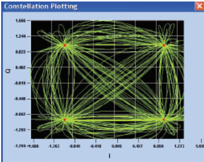
Figure 2. Expanded view of a QPSK constellation.
