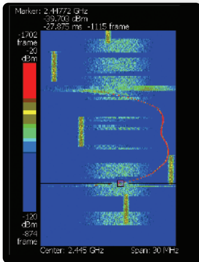
► Figure 11. This spectrogram reveals two common spread spectrum signals. The yellow hopping signal is a Bluetooth FHSS transmission, while the constant center frequency aqua signal is a WLAN DSSS transmission. The red line is caused by a microwave oven leaking RF radiation.
