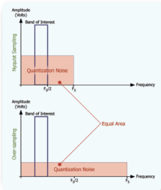
► Figure 21. Increasing the over-sampling rate spreads out the quantization noise, lowering the noise floor.
