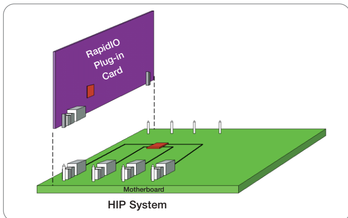
► Figure 1. HIP Architecture.
