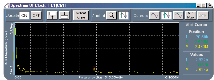
► Figure 10. Jitter Spectrum.
