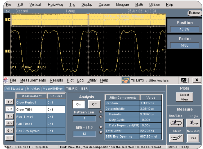
► Figure 12. TDSJIT3 reports the estimated eye opening at the specified BER level and breaks down its random deterministic components.
