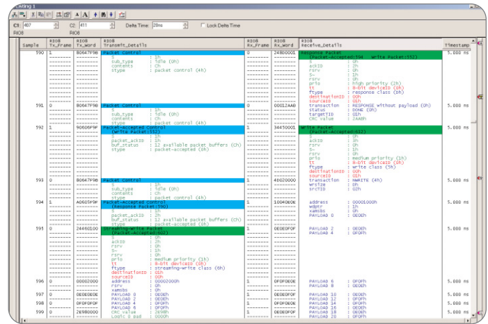
▶ Figure 7. Illustration of a packet-style view of captured data from a RapidIO protocol using a listing window.
