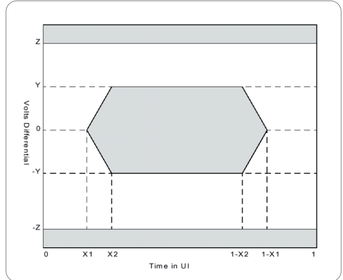
► Figure 15. Example of an eye diagram mask defined in differential voltage and Unit Interval.
