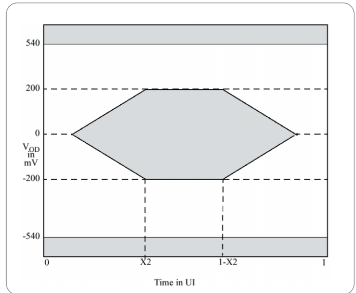
▶ Figure 13. RapidIO Transmit Mask
