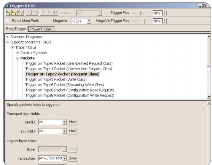
► Figure 6. Example of Easy Trigger.
