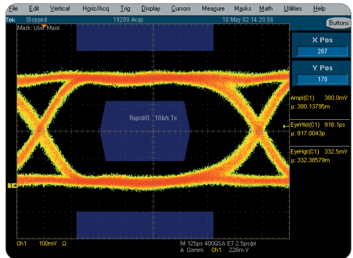
► Figure 16: Actual RapidIO 1Gb/s Tx signal captured with a real-time oscilloscope. It passes the mask test.
