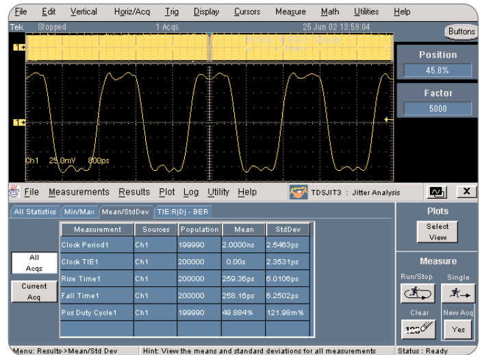
▶ Figure 11. Real-time oscilloscopes permit analysis of cycle-cycle jitter effects.
