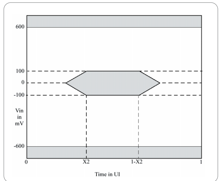
▶ Figure 14. RapidIO Receive Mask
