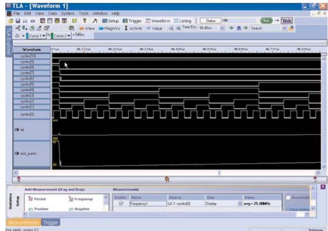
▶ Figure 8b. TLA Series logic analyzer automates and simplifies many measurements.
