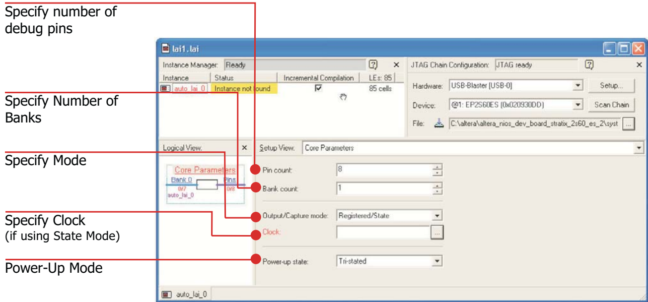
▶ Figure 3a. Example of Altera's Logic Analyzer Interface Editor used to define and insert test core.
