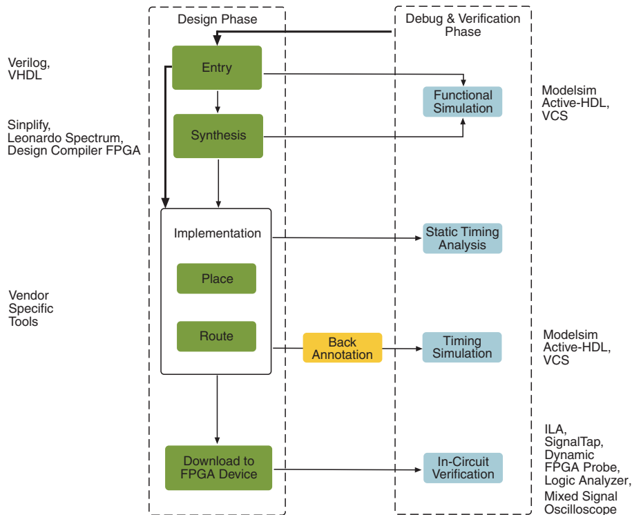
▶ Figure 1. FPGA Design Flow.
