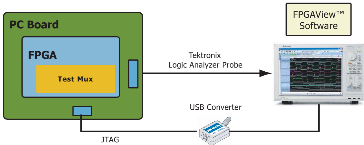
► Figure 2. Typical FPGAView implementation.
