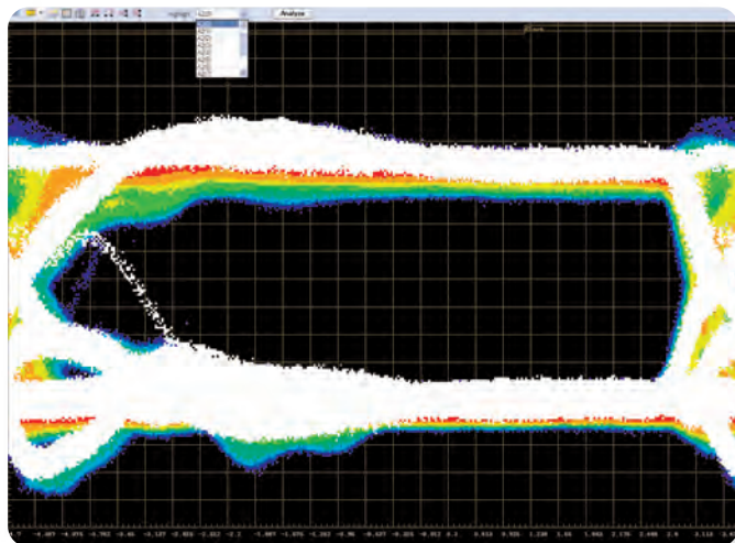
► Figure 5. On this oscilloscope-generated eye diagram, white highlights show a cross talk problem caused by the A2 (0) signal.
